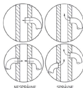
Fig. 1 Connection to the chimney incorrect correct
