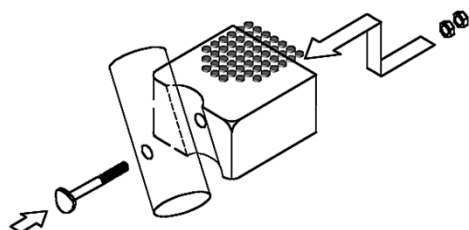
Detail X
