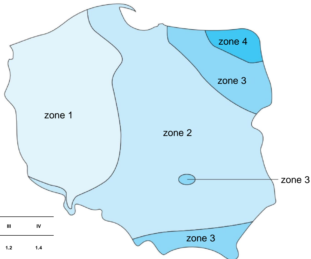
Ground frost zones
