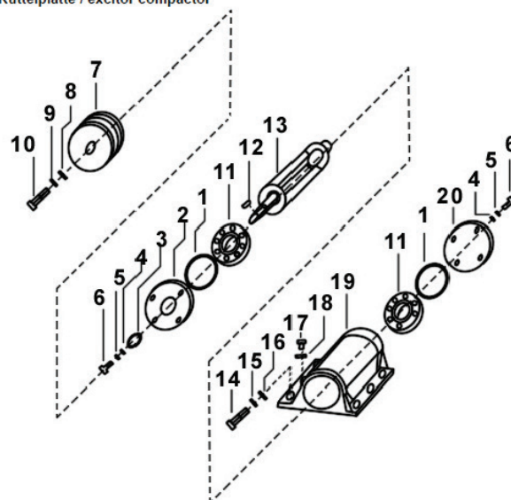
Erreger Rüttelplatte / excitor compactor
